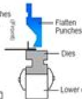
Flatten kneebend (carry out) Plate thick: 0.4~3.2mm
