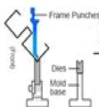
90° Kneebend (Frame) Plate thick: 0.4~2.3mm
