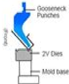
90° Kneebend (Gooseneck) Plate thick: 0.4~5.0mm
