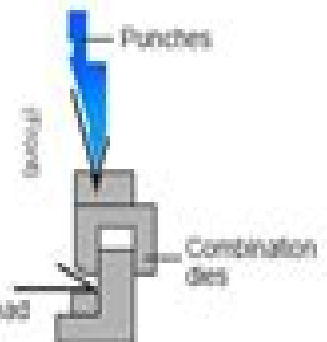
V&Flatten kneebend Plate thick: 0.4~1.6mm
