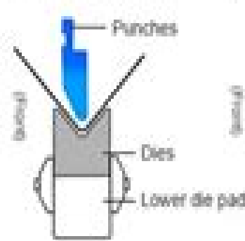
90° Kneebend (Thick plate) Plate thick: 4~10mm
