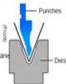
Acute angle (Thick plate) Plate thick: 4~5mm
