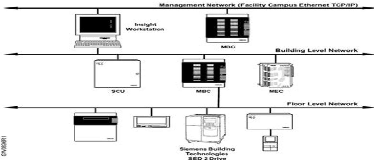
Figure 1. System Architecture.
