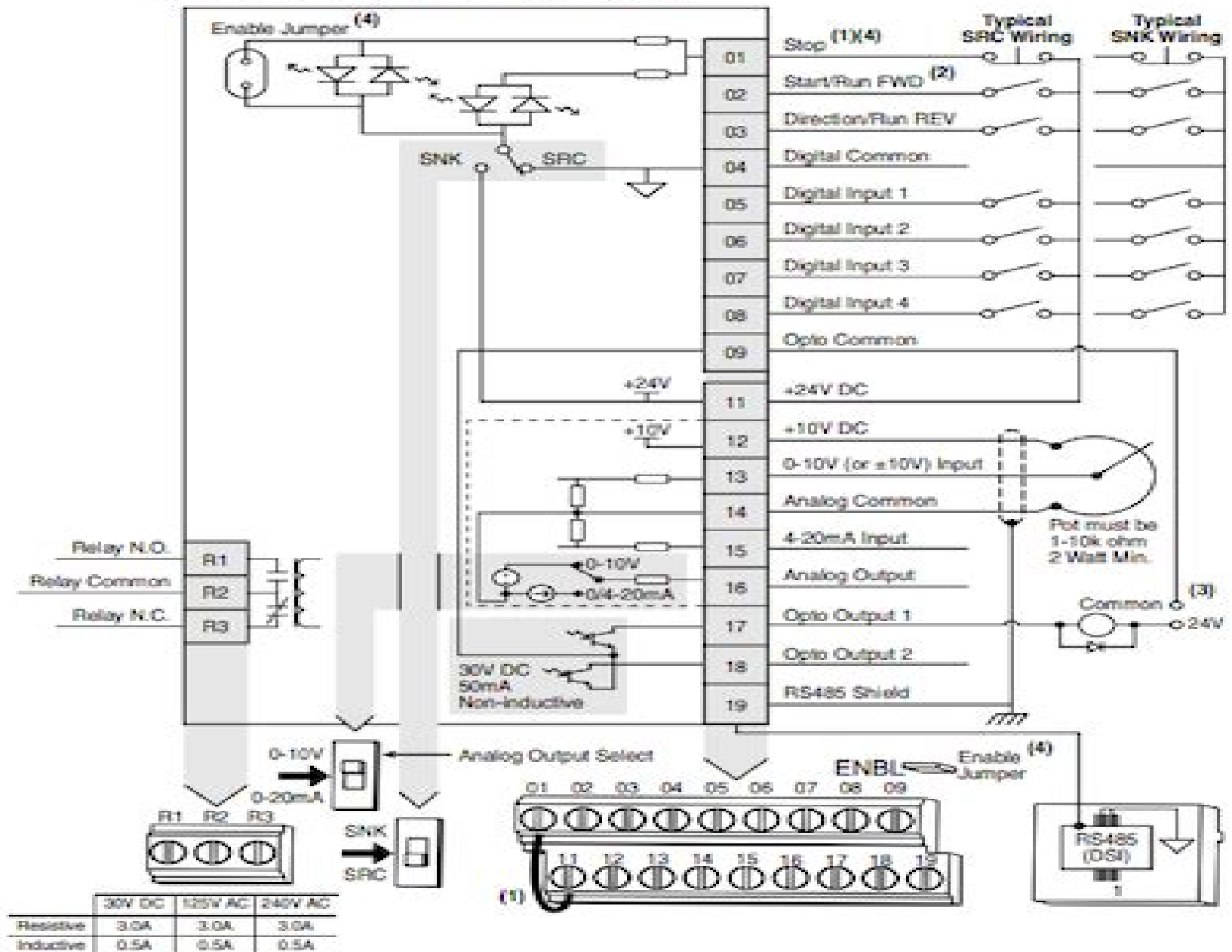
Figure 1.5 Control Wiring Block Diagram
