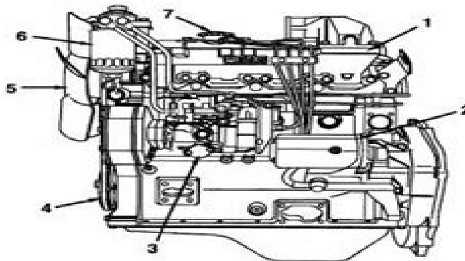
Intake Side (Naturally Aspirated)
