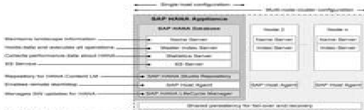
SAP HANA System Example Deployment Architecture
