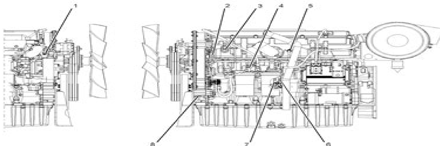
Illustration 5 Locations of the sensors on the 2506-15 engine
