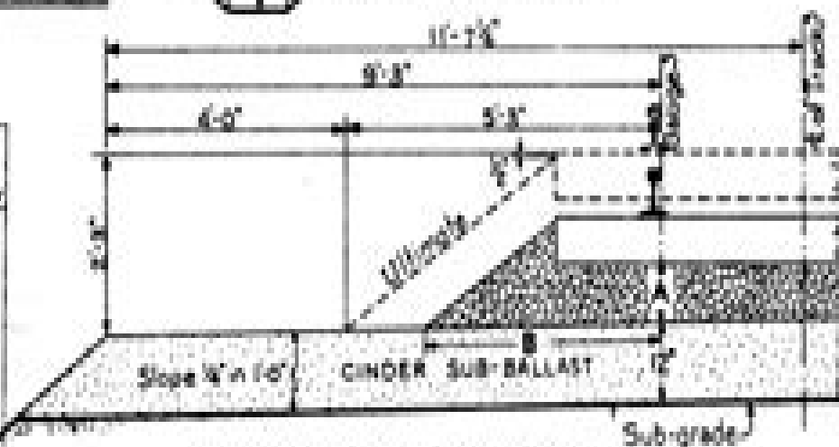
SECTION OF ROADWAY ON FILLS
