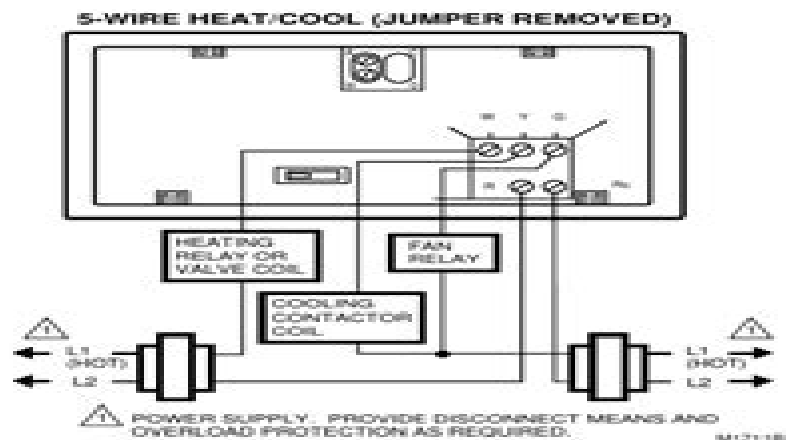
Fig. 8. 5-wire heat/cool application (jumper removed).
