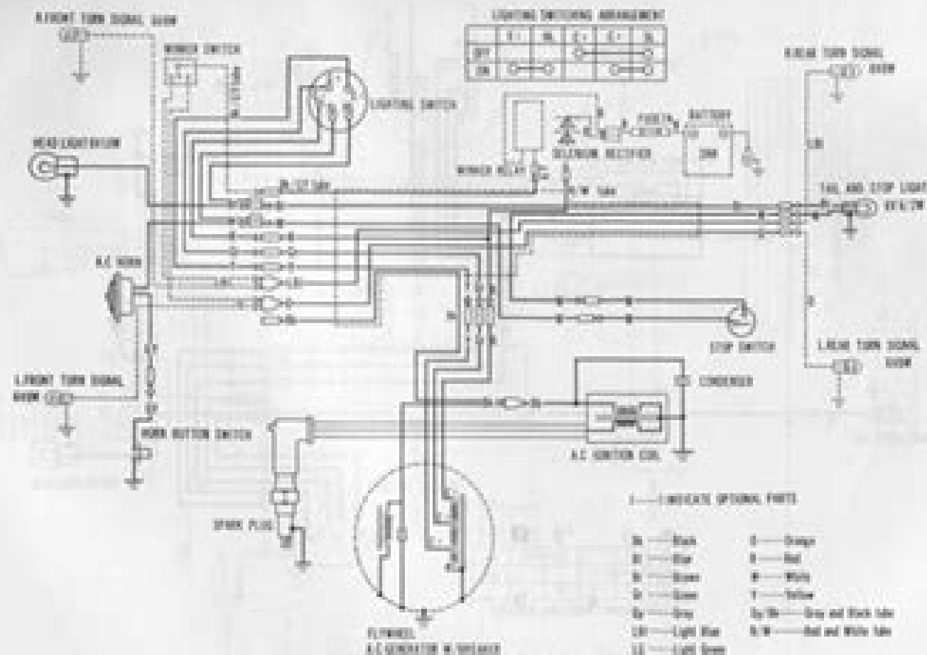
PC 50 WIRING DIAGRAM (General export type)
