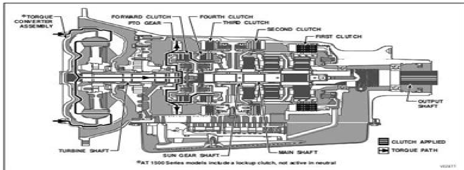
Figure 2-1. Neutral Power Flow
