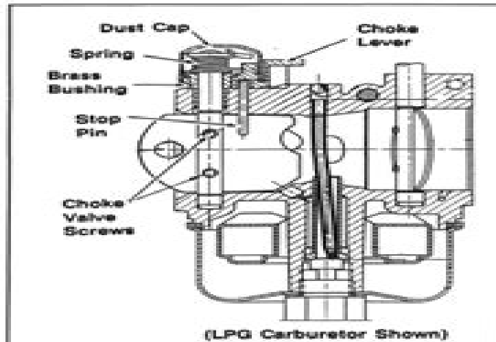
Figure 5-12. Cutaway View Showing Self-Relieving Choke Carburetor.
