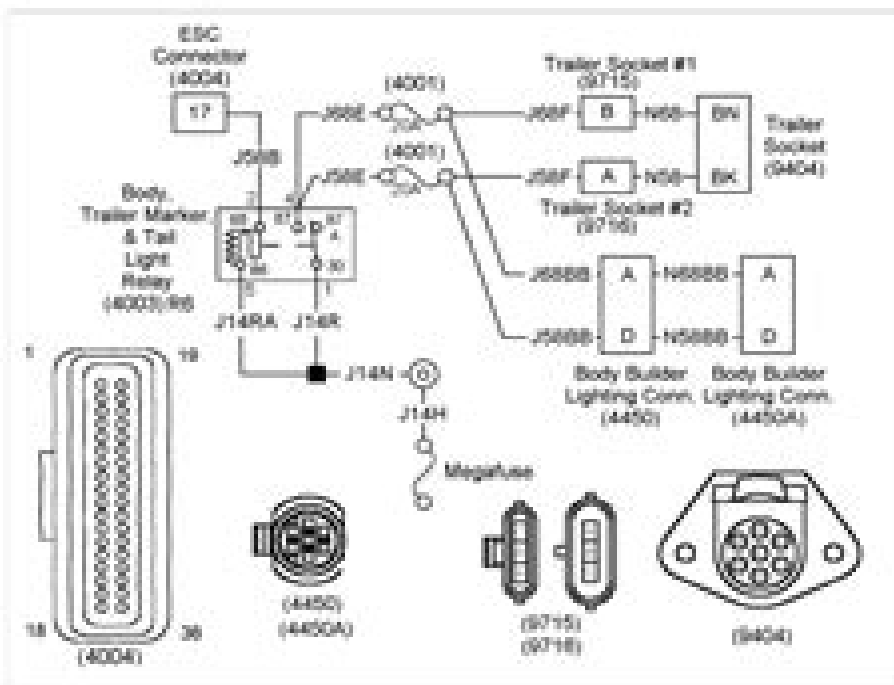
Figure 5-49 Body, Trailer Marker & Tail Light Relay Circuits—Always Refer To Circuit Diagram Book For Latest Circuit Information
