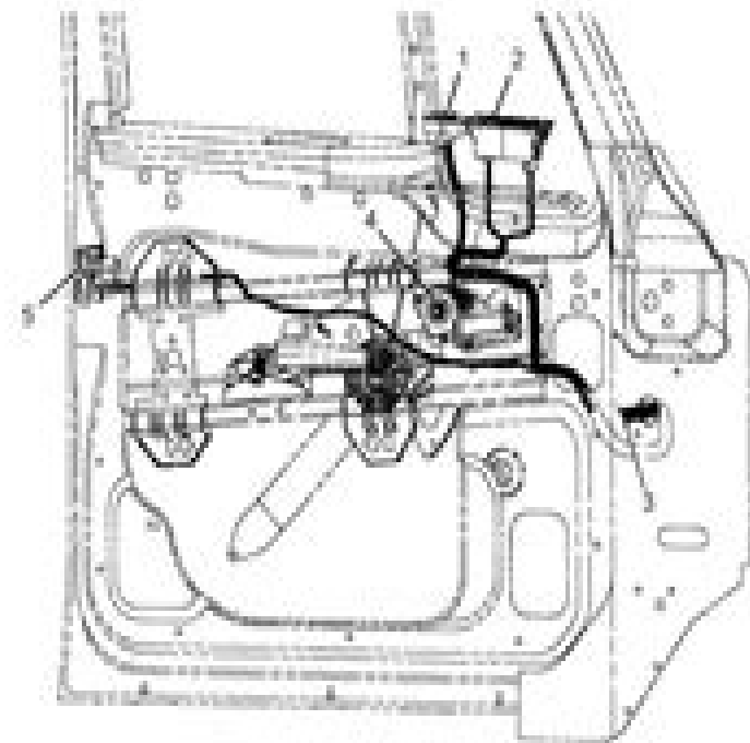
Figure 210 Power Window and Lock Wiring (Driver's Side Shown)
