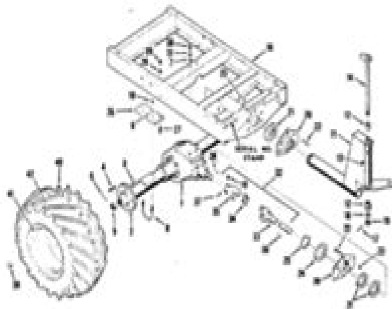
ILLUSTRATION 1 REAR FRAME & DRIVE LINE
