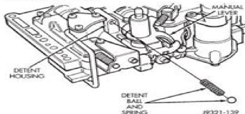
Fig. 94 Detent Ball And Spring Removal
