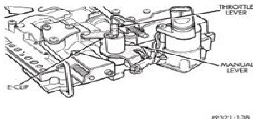
Fig. 93 Removing Throttle Lever E-Clip
