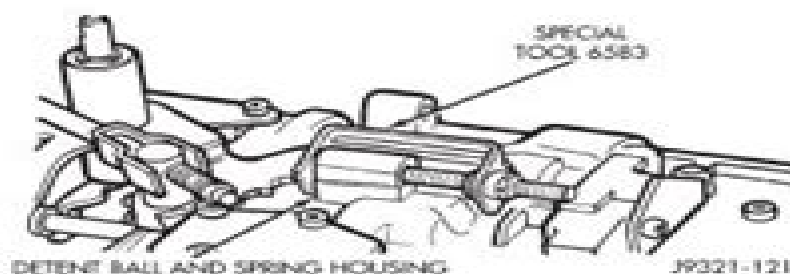
Fig. 92 Securing Detent Ball And Spring
