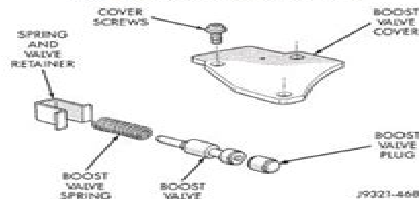
Fig. 91 Boost Valve Components
