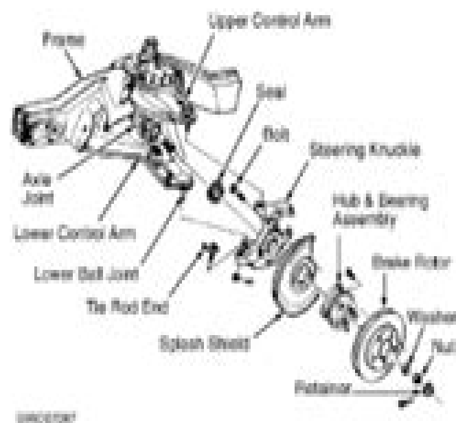
Fig. 1 Exploded View Of Hub & Steering Knuckle Assembly ("T" Series Shown; "K" & "L" Series Are Similar)
