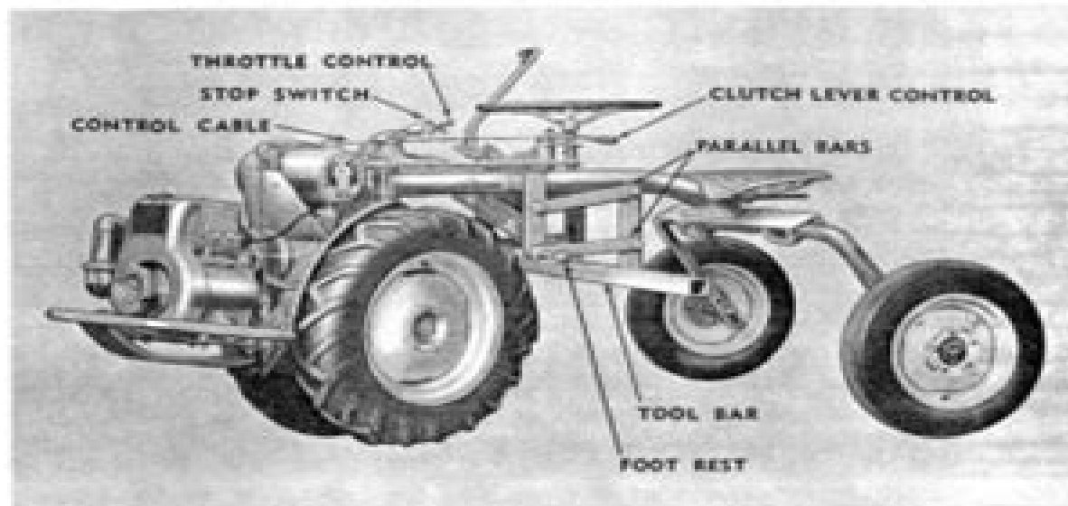
Figure 1. Bolson Sidemaster - Left Front View
