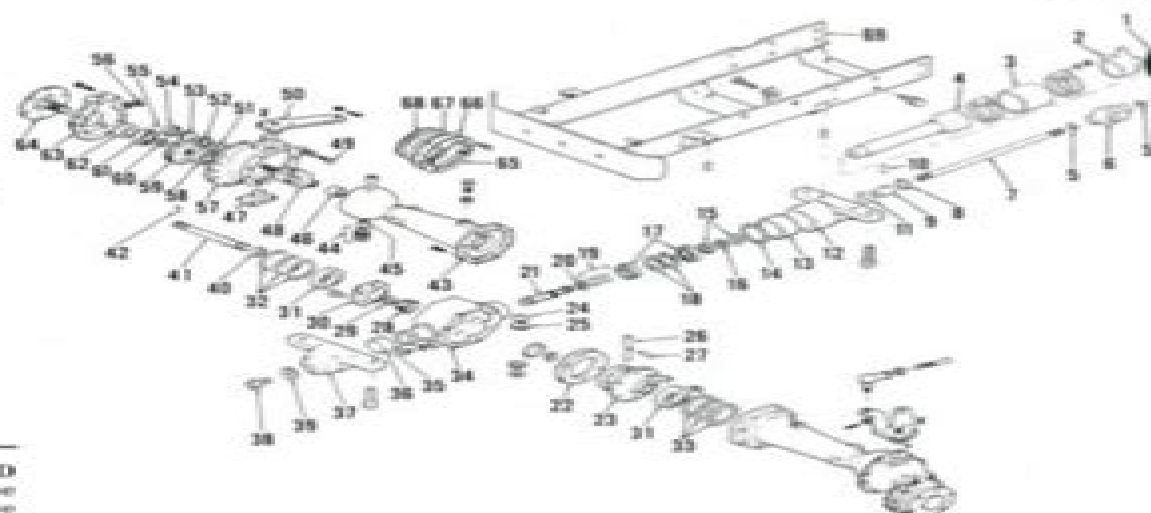
Fig. 7—Exploded view of front wheel drive axle used on 1100 and 1200 models.
