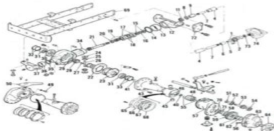
Fig. 8—Exploded view of front wheel drive axle assembly used on 1300 models.
