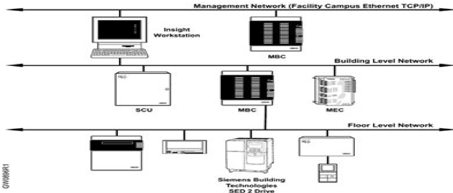
Figure 1. System Architecture.
