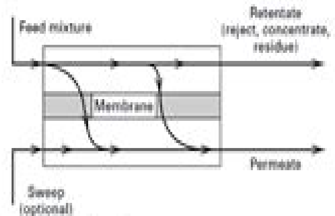
Figure 14.1 General membrane process.
