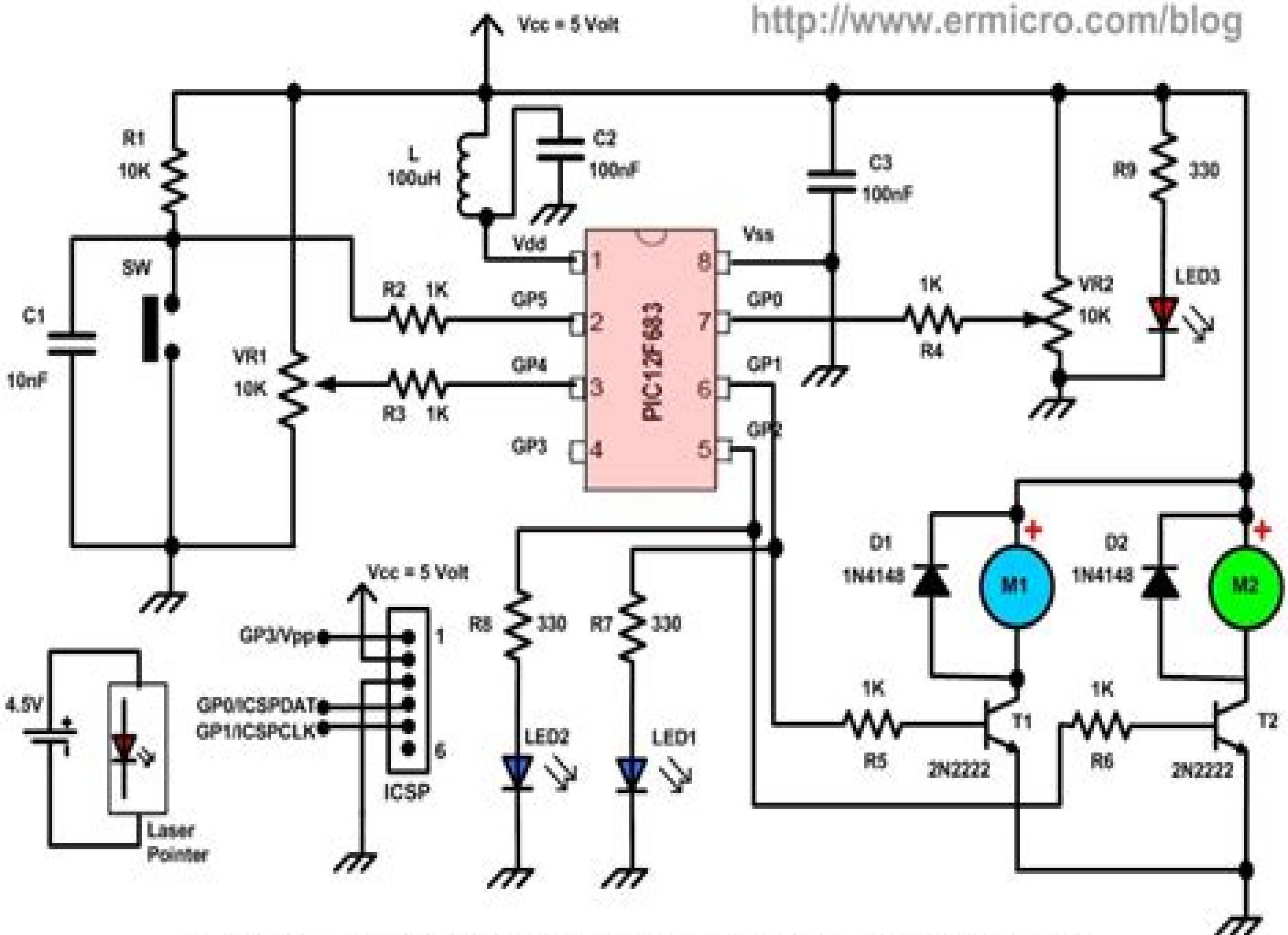
The Laser Projector Schematic using the Microchip PIC12F683 Microcontroller
