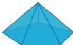
Pentagonal pyramid
