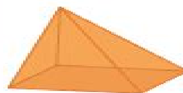
Rectangular pyramid
