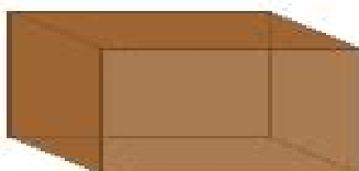
Square prism
