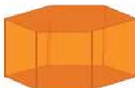
Hexagonal prism
