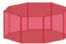
Octagonal prism
