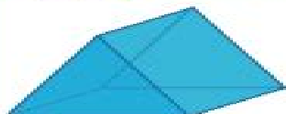
Triangular prism
