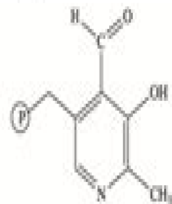
Pyridoxal 5'-Phosphate
