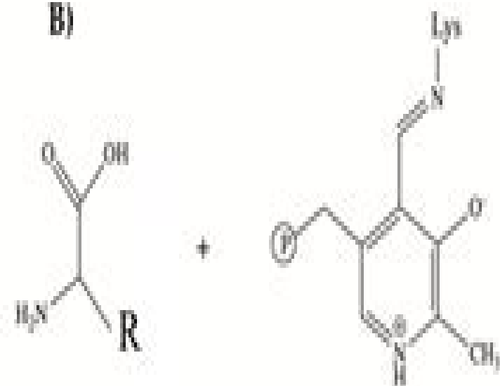
Internal Aldimine
